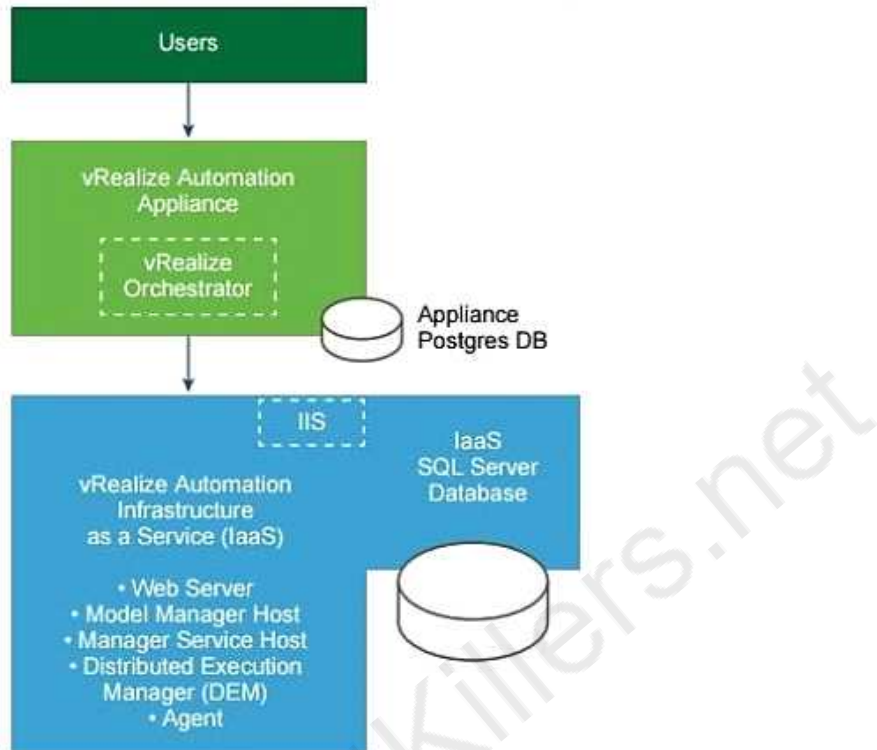
Figure 1-1. Minimal vRealize Automation Deployment
